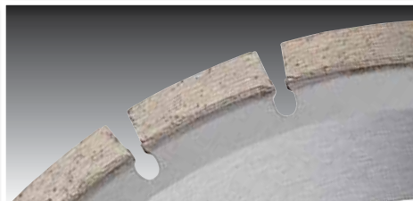
Anti-crack gullets help prevent core cracking.
